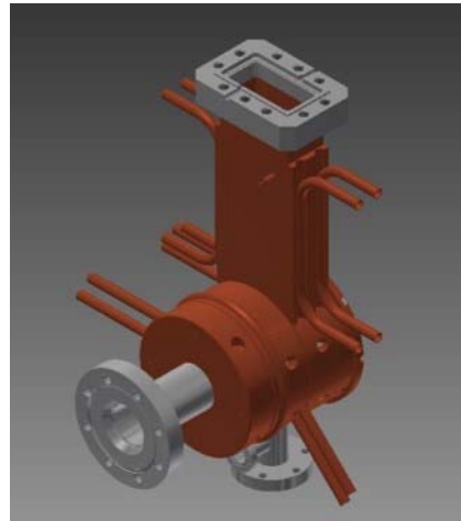
Figure 4: New high-repetition-rate RF gun.
