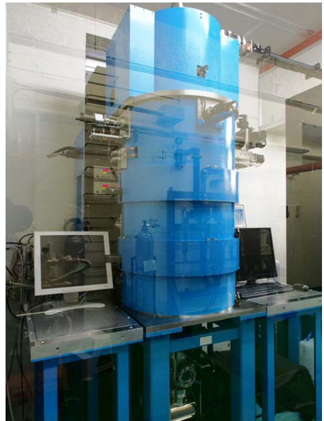
Figure 3: Photo of time-resolved relativistic-energy electron microscopy using RF gun
