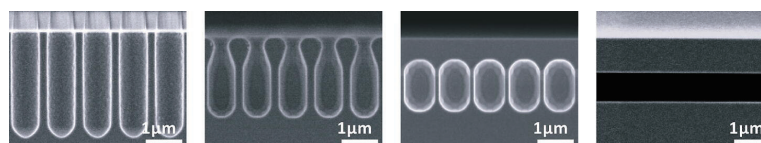
Surface-diffusion-driven evolution of a hole pattern on Si
