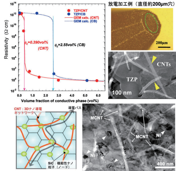
Percolation characteristics of electrical resistivity for ZrO_2/CNT nanocomposites, their microstructure and 1D/0D/ceramic multi-phase nanocomposites.
